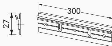
Inhaakprofiel
